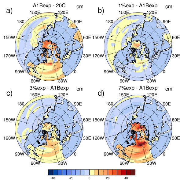
Figure 3. Dynamic sea level anomalies: (a) the mean of 2080–2099 in A1Bexp minus the mean of the last 20 years of the 20th century; (b–d) are the mean of 2080–2099 in 1%exp, 3%exp, and 7%exp minus the mean of 2080–2099 in A1Bexp, respectively.
