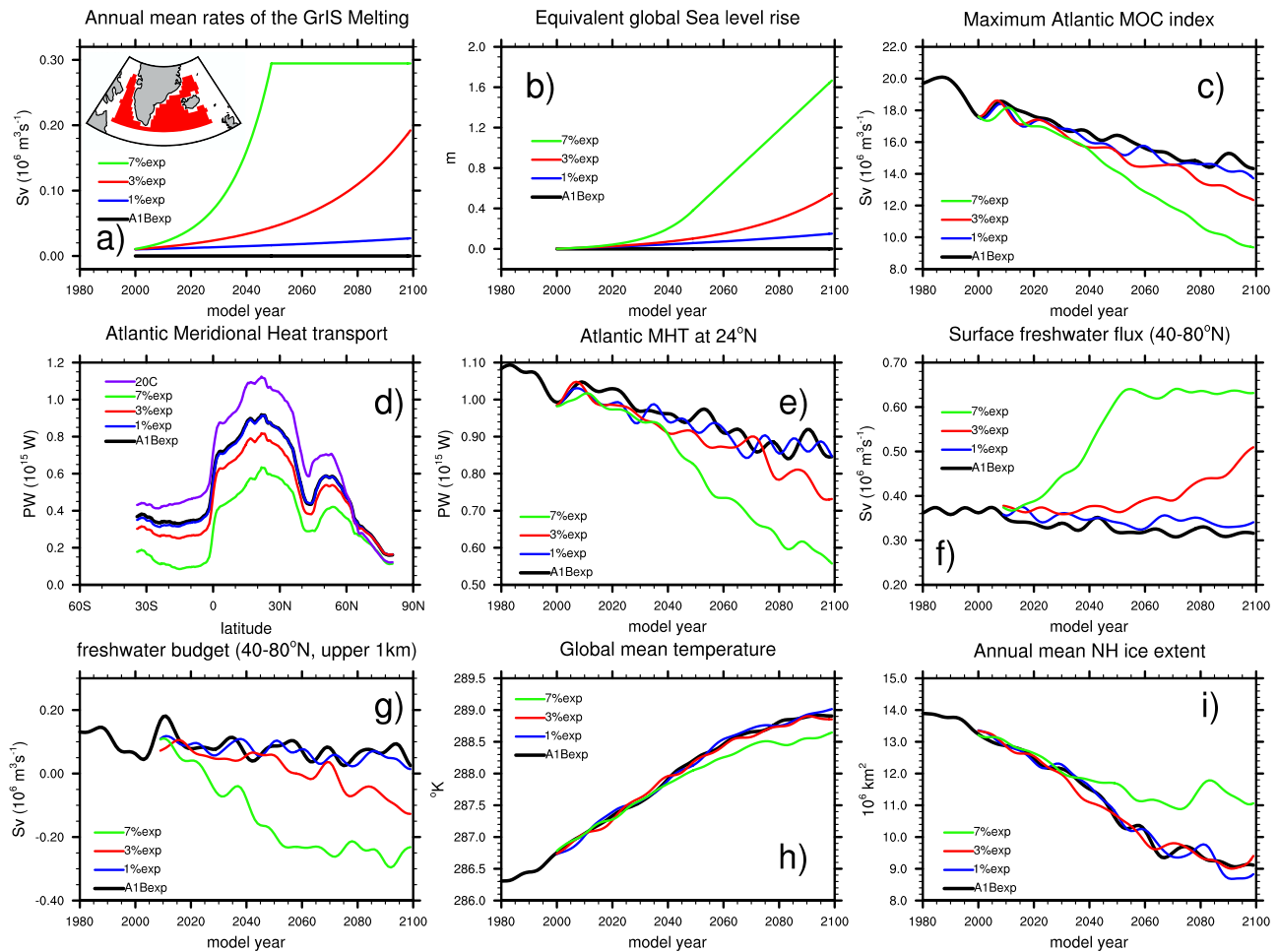
Figure 1. (a) Time evolving annual mean rate of the GrIS melting in the experiments and (b) the equivalent cumulative global sea level rise due to this melt flux. (c) Changes of the MOC index, (d) the annual mean Atlantic meridional heat transport averaged over 2080–2099 for 21st century runs and averaged over 1980–1999 for the 20th century run and (e) changes of this transport at 24°N, (f) changes of the surface freshwater input (positive represents oceanic freshwater gain) and (g) the freshwater budget for the upper 1000 meter of the North Atlantic (40–80°N, positive represents oceanic freshwater loss), (h) the global annual mean surface temperature, and (i) the annual mean Northern Hemisphere sea ice extent. The insert in Figure 1a shows the region where the Greenland melting is uniformly added into the model.
