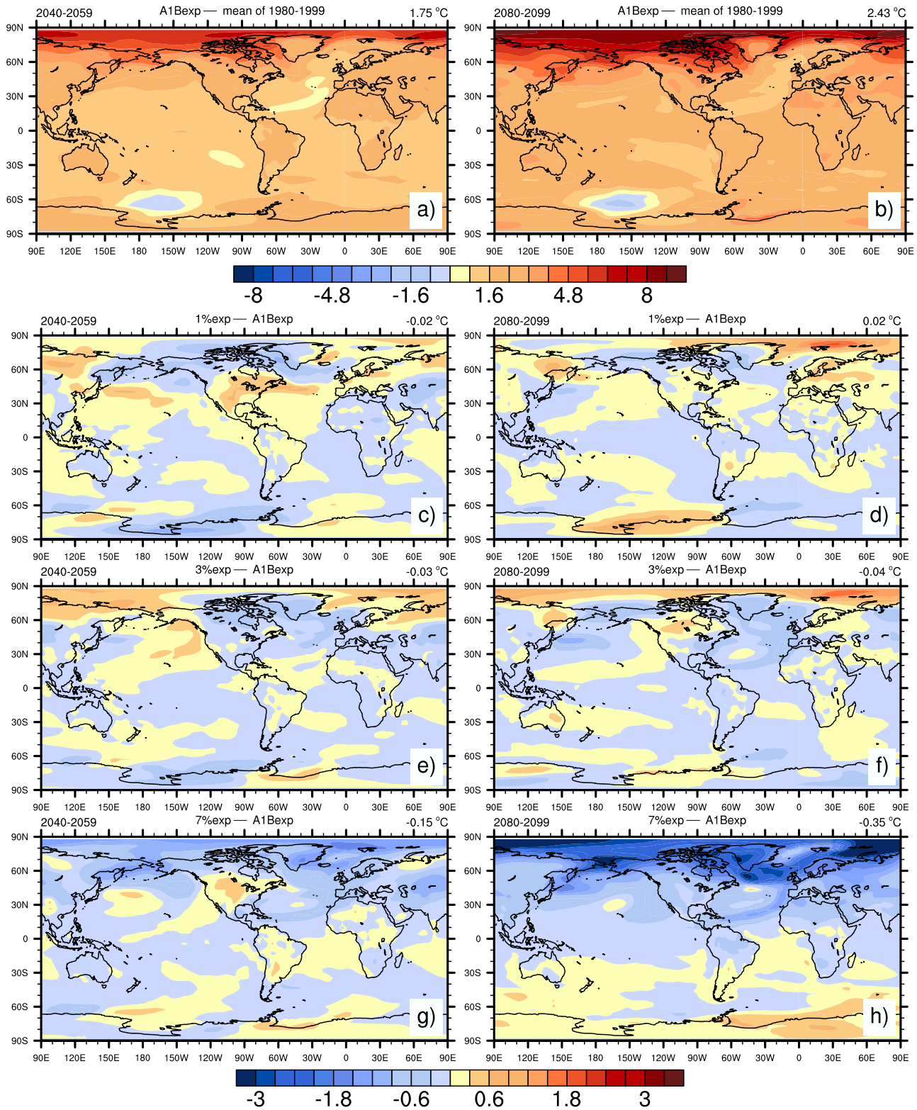
Figure 2. 20-year mean surface temperature anomalies: (a and b) are the temperature anomalies in the A1Bexp relative to the late 20th century (1980–1999); (c–h) are the temperature anomalies of the sensitivity simulations relative to the standard A1Bexp in (left) the mid-21st century and by (right) the end of the 21st century.
