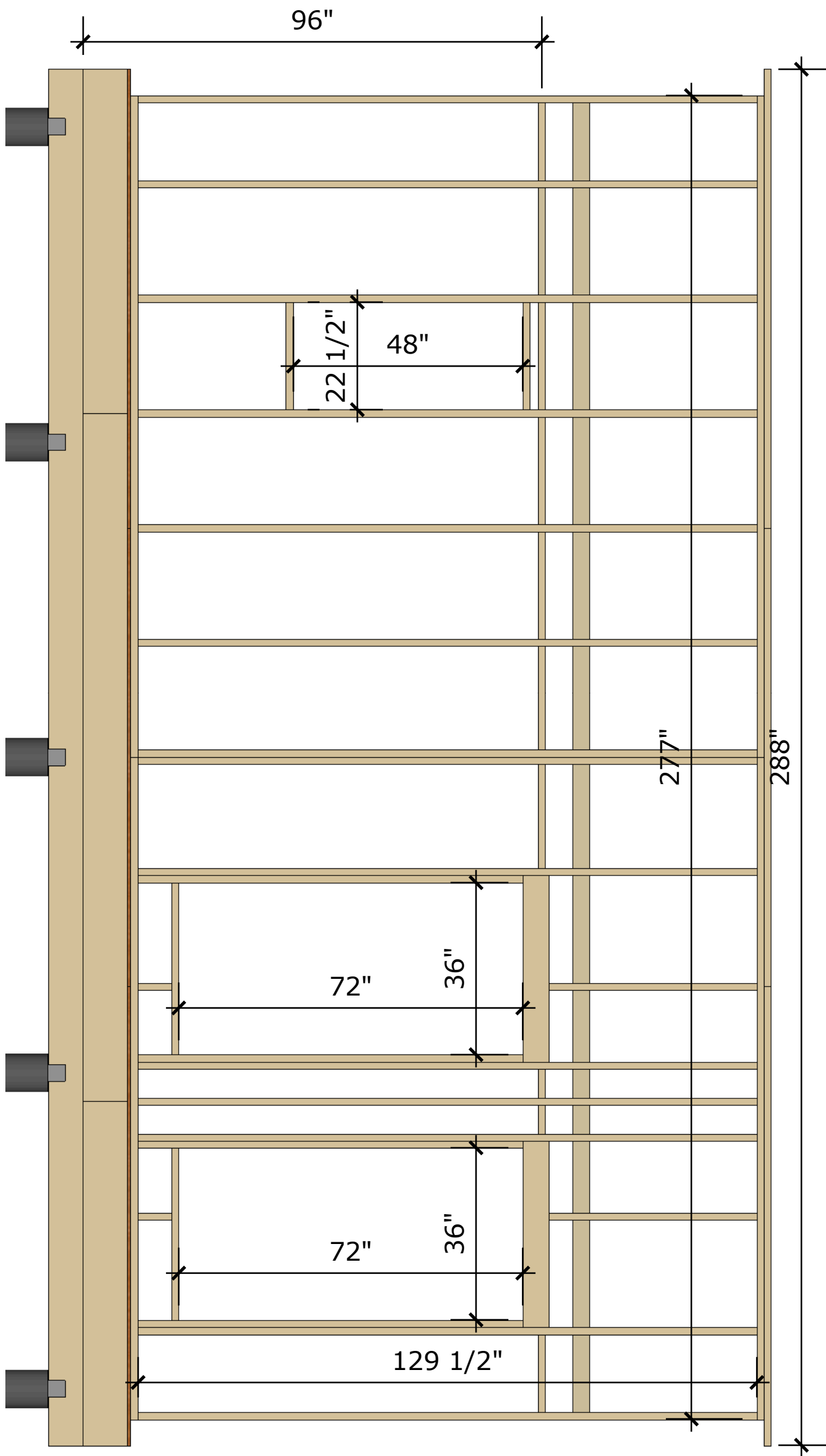
Left Wall Framing
