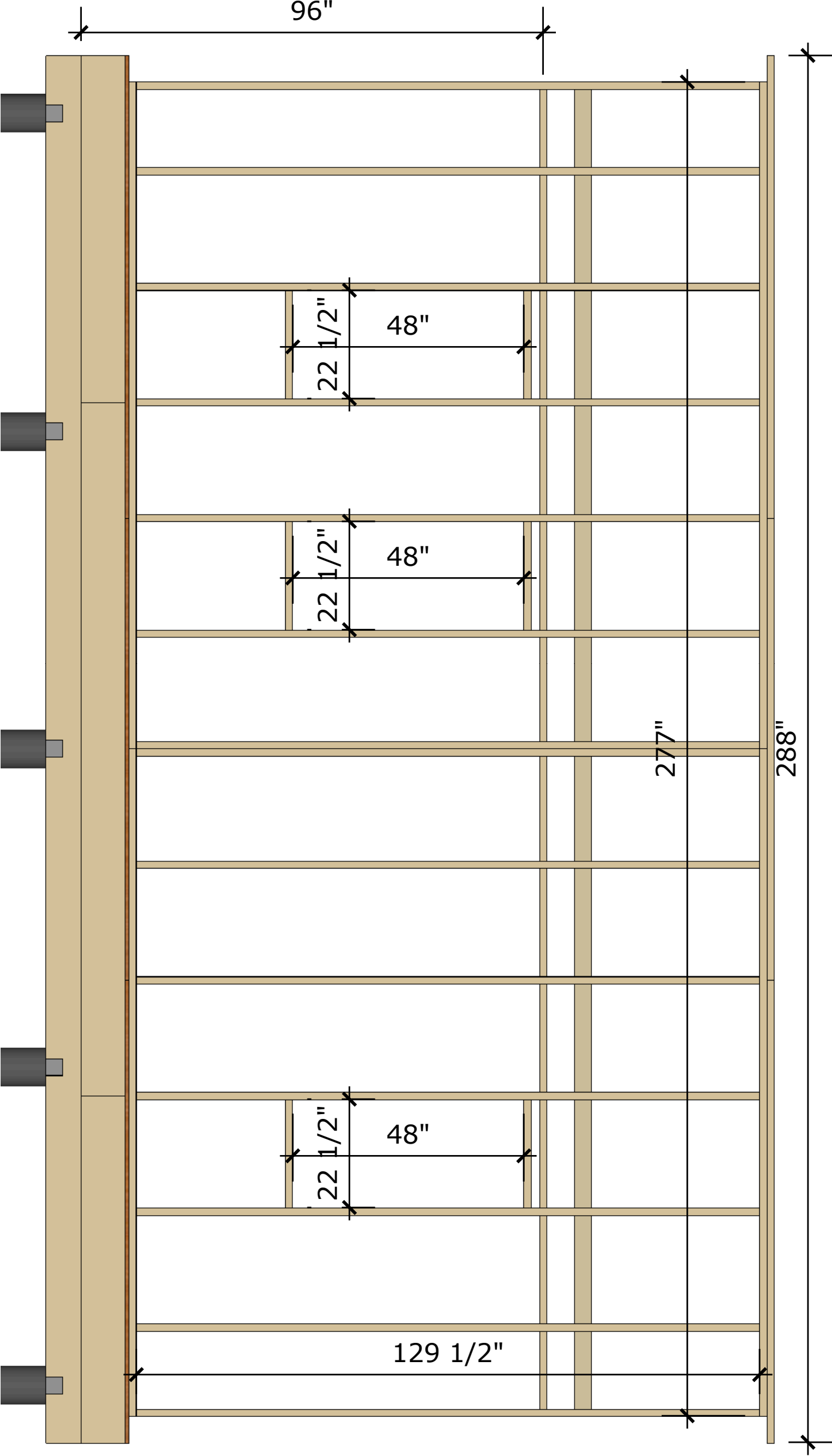
Right Wall Framing
