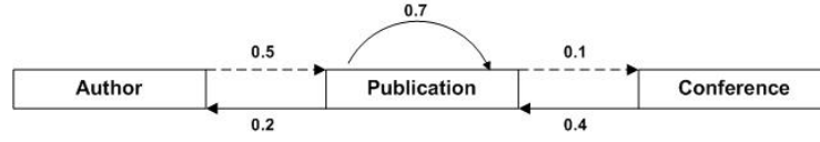
Fig. 5. Authority transfer annotation ontology for a publication ontology
