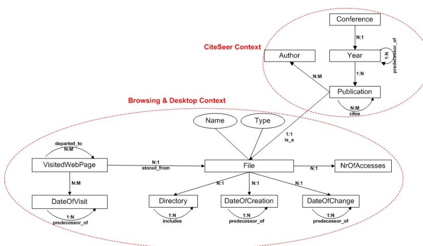
Fig. 3. Context ontology for our prototype
