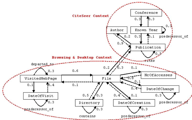
Fig. 4. Authority transfer annotations, including external ranking sources
