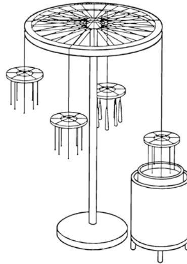
Figure 4: Dipping equipment
