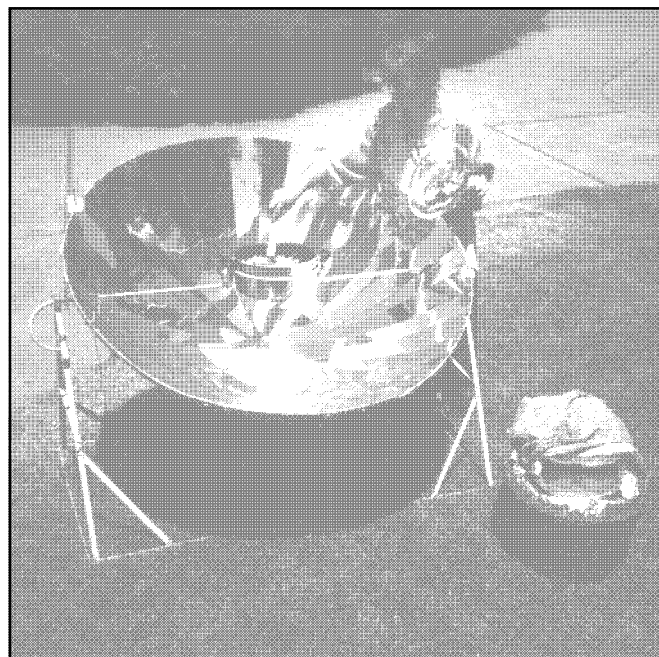
Above: The SK 12 solar cooker at work on ratatouille. Note the haybox basket used to keep the food hot while the next pot is placed in the cooker.
