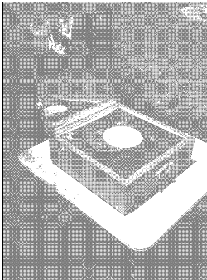
Above: This variation of the Kerr-Cole design allows access to the food without opening the box and allowing heat to escape.
