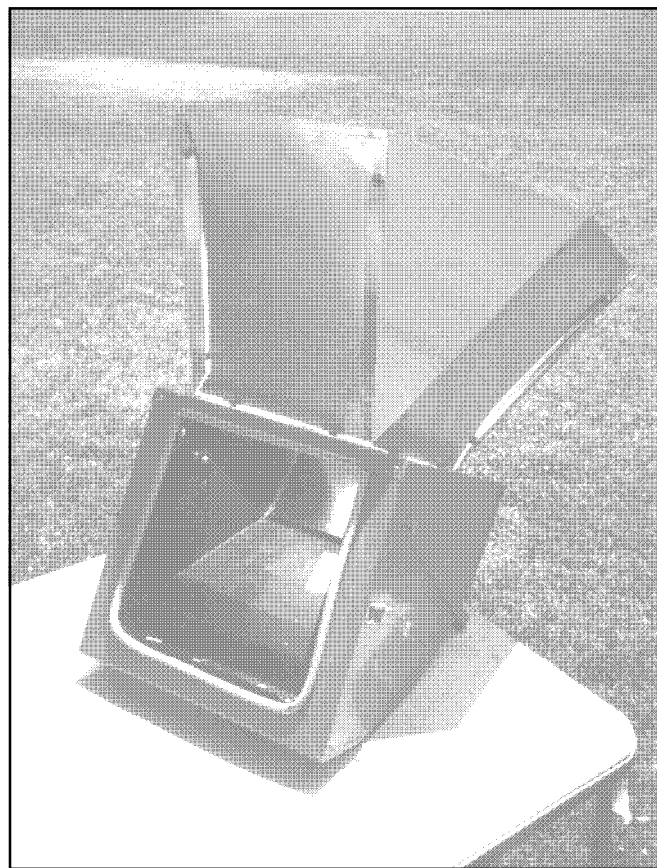
Above: The tray on which the pot rests is suspended, so that the pot always stays level. This design also allows access to the food from the back.
