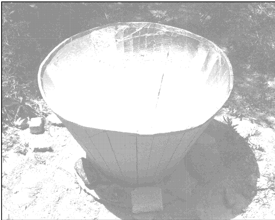
Above: Jay Campbell's cooker won first place. Photo by Jay Campbell
