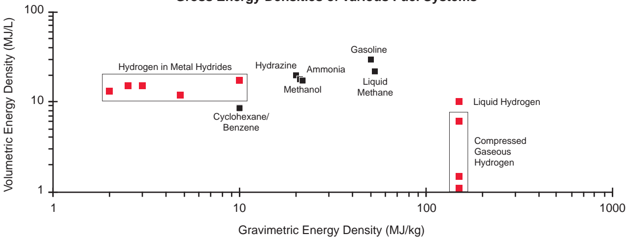
Gross Energy Densities of Various Fuel Systems
