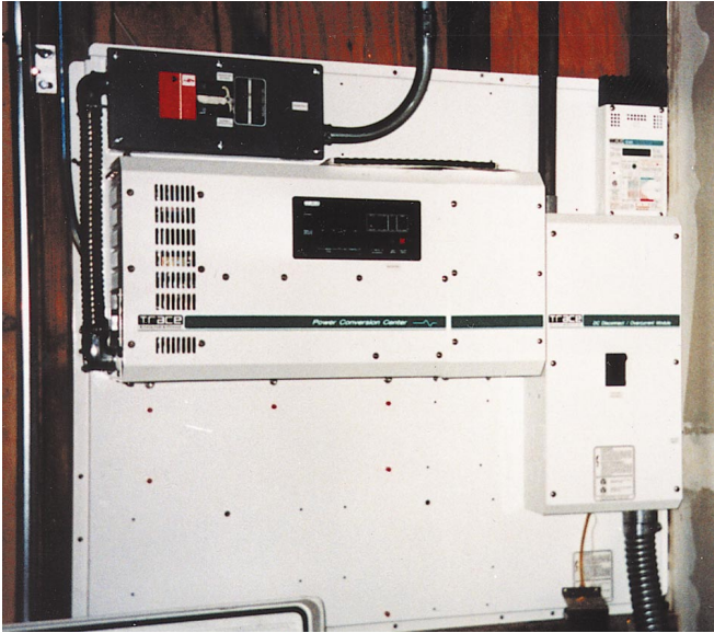
Above: Trace PP-22SW4024 Power Panel with SW4024 inverter, C-40 charge controller, DC-250 Heinemann circuit breaker, and 60 amp bypass breaker set.
