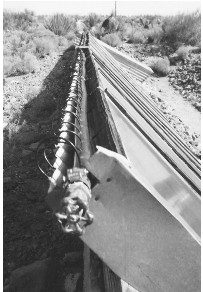
Above: Top view of solar collectors showing the water manifold.
