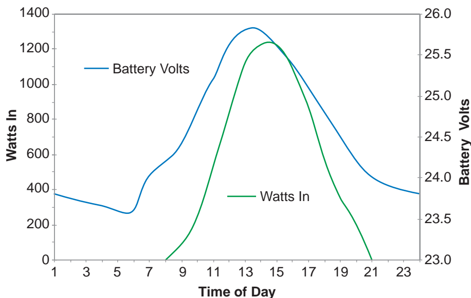
Graph 2: Input Watts vs Battery Voltage
