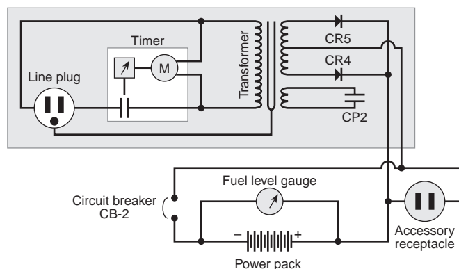
Figure 1: E10 Charger Circuit
