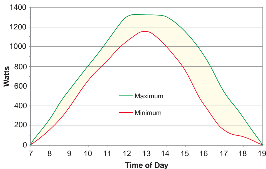
Graph 1: Minimum & Maximum Input Watts
