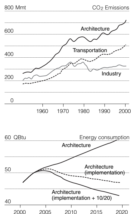
Fig. 11a, b: In the U.S., "architecture", which includes all residential and commercial sectors, along with the portion of the industrial sector containing buildings and building materials, is the largest single energy user (at 48 % of primary energy), as well as the largest, and fastest growing, emitter of CO 2 . Aggressive but totally achievable (and affordable) changes in buildings efficiency policy nationwide could lead to a reduction in building energy use, shown as the "implementation" trajectory in the lower graph. If the Union of Concerned Scientist's "Clean Energy Blueprint" is also adopted (10 % of U.S. electricity from renewables by 2015 and 20 % by 2025) the energy impact of buildings in the U.S. could be further reduced as shown in the "implementation + 10/20 portion" of the graph. Source: Edward Mazria, SOLAR TODAY, May/June, 2003, 48-51
