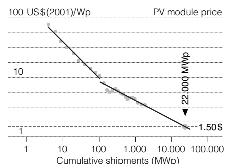
Fig. 15b: PV experience curves for 1976-2001 and projection to a breakeven price of US$ 1.50/W p , demonstrating the importance of promoting high volume applications. Slide source: Dr. John Byrne, data by Paul Maycock (2002)
