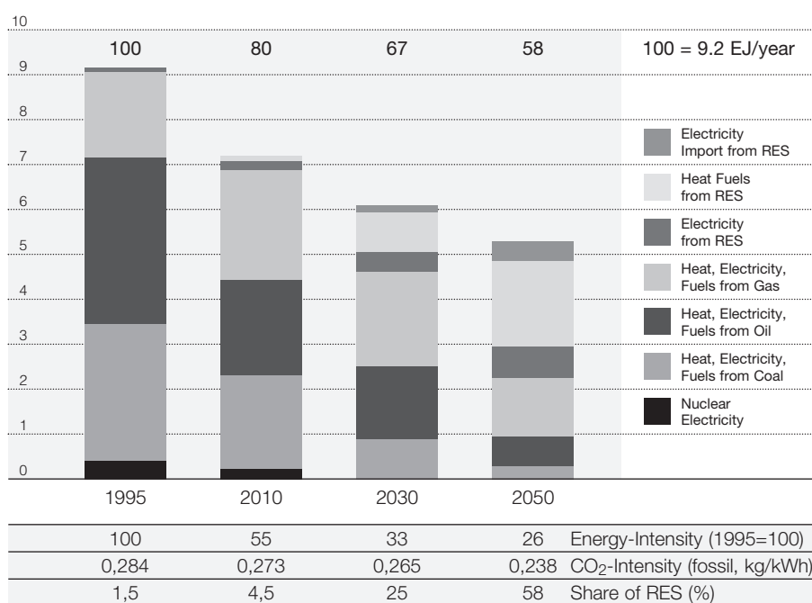
Fig. 19: A plausible long-term German plan to reduce energy use in an expanding economy, and to bring renewable energy use up to significant percentage levels
