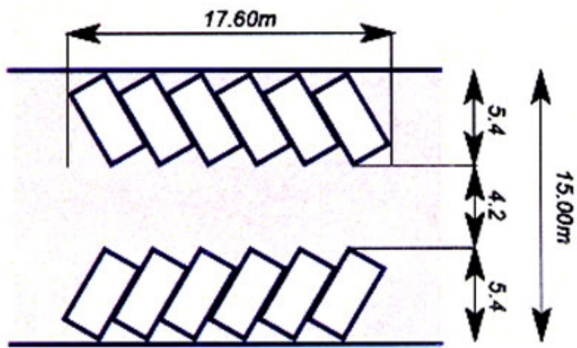
60° Parking
