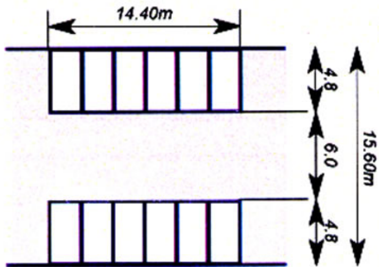
90° Parking
