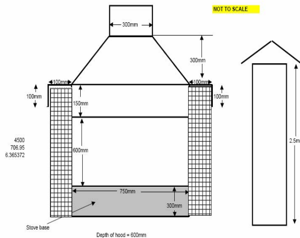
Figure 5: Stove dimensions used in the Tanzania smoke hood.
