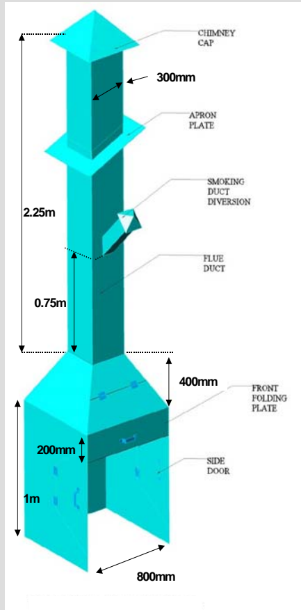
Figure 6: Nepal smoke hood.
